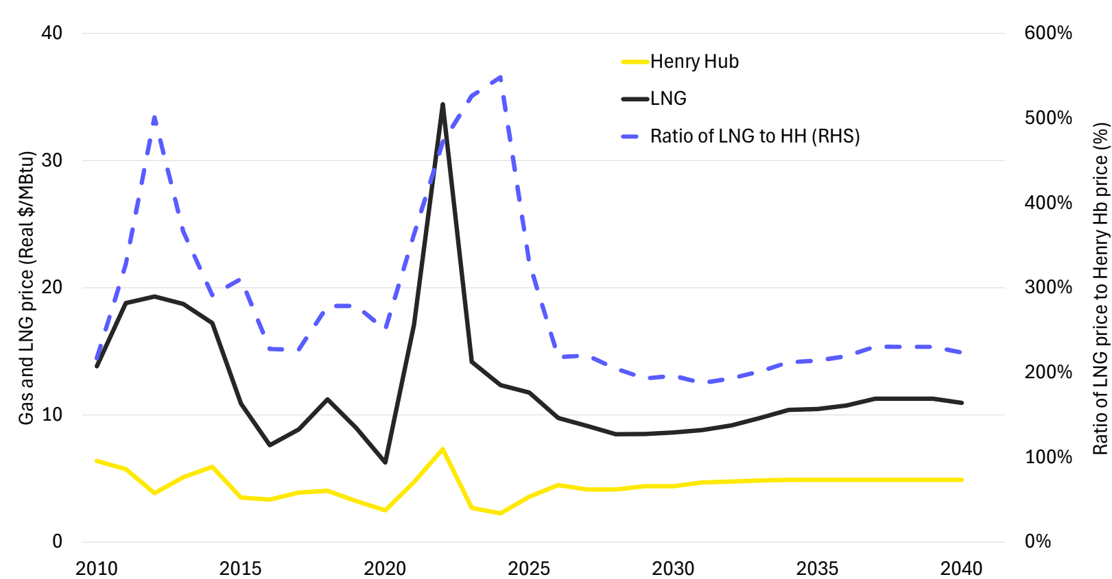
LNG 1 is between two and five times the cost of US pipeline gas
